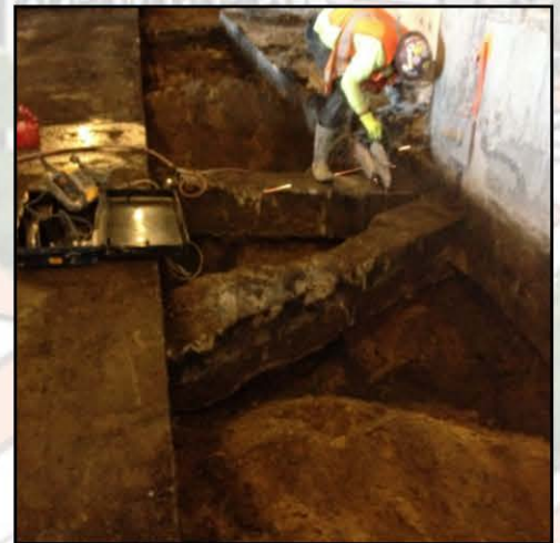
11/2014 The last step in preparation for the demolition of the former baggage building was the cutting of the grade beam ties to the retaining wall for the rail lines.
